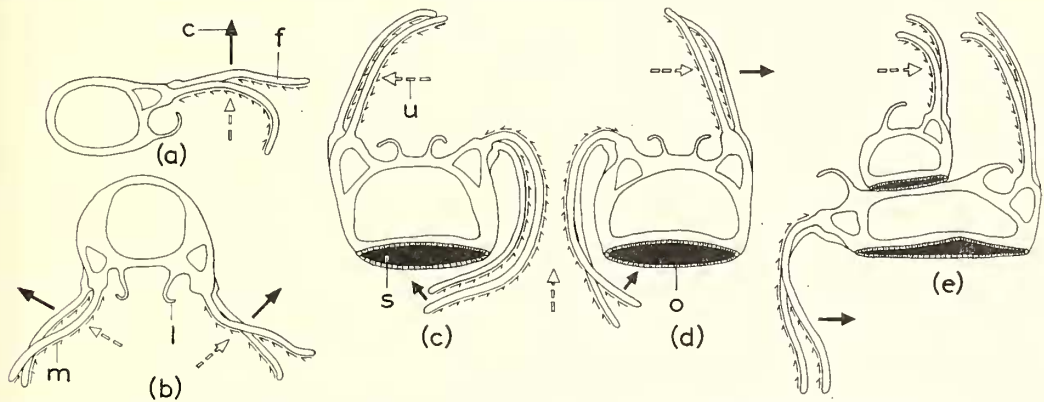
TEXT-FIG. 12. Transverse sections through the spirolophe of Tegulorhynchia (a) and the side arm of Terebratulina (b) and the inferred deuterolophe of spiriferoids (c), (d), with accessory calcareous spires (e):—f. filament, l—brachial lip, m—direction of movement of food particles, o—outer epithelium, s—supporting calcareous ribbon, u—unfiltered, inhalant current, c—filtered, exhalant current.
